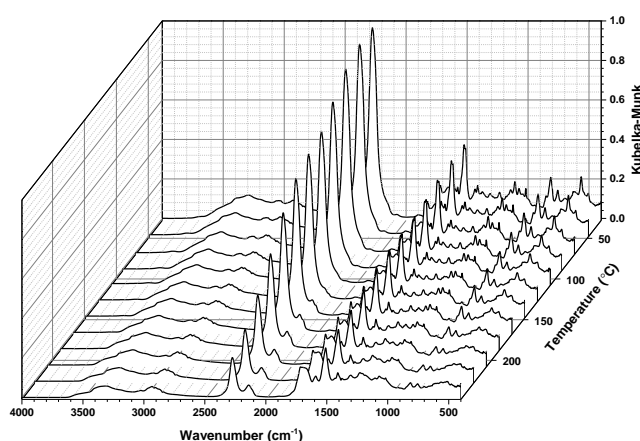
In-situ DRIFT spectra presenting the curing evolution of pMDI with soy protein.
