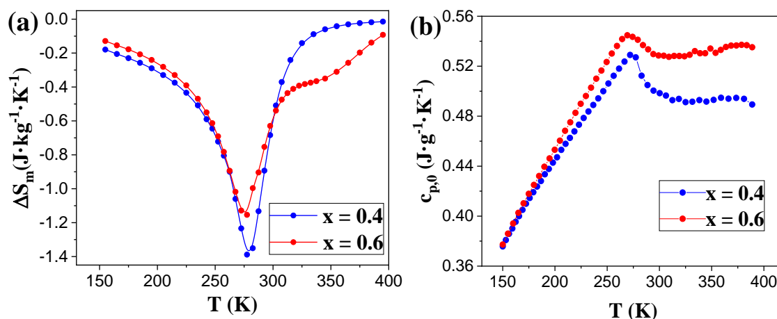
Figure 1: Temperature dependence of \Delta S_m(\mu_0 H = 1.5 T) (a) and specific heat c_{p,0}(\mu_0 H = 0 T) (b) for x = 0.4 and 0.6 samples milled for 100 h.
