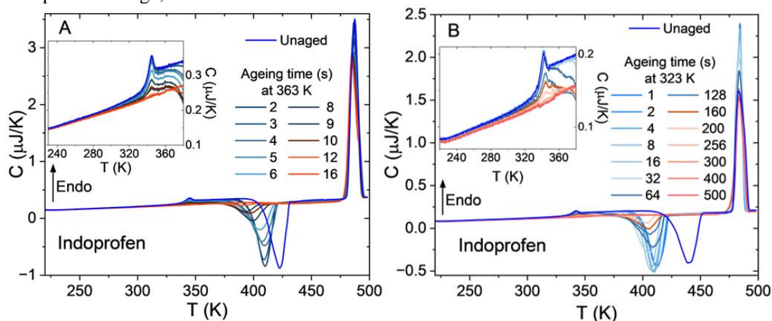
Fig. 1. Isothermal crystallization of indoprofen after cooling at 300 K/s from the liquid state to the crystallization temperature, probed by reheating at 300 K/s from the glassy state. Panel A: crystallization at 363 K ( \sim T_g+30 K) at different times. Panel B: crystallization at 323 K ( \sim T_g-10 K) at different times. Insets: detail in the glass transition region.
