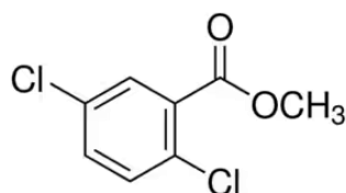
Methyl 2,5-dichlorobenzoate
