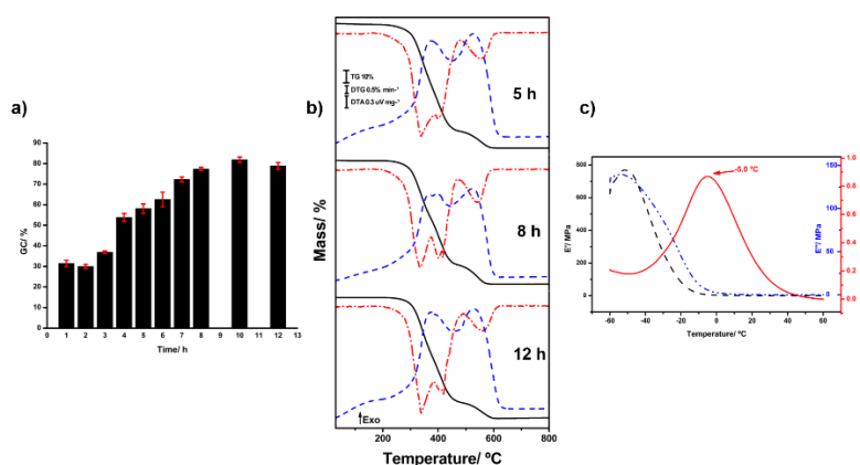
Figure 1- a) Gel content evaluation caption of polymerization, b) TG/DTG-DTA curves and c) Storage ( E' ), loss ( E'' ) modules and \tan\delta curves.
