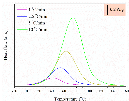
Figure 2. Exothermic curing curves under different heating rates by means of DSC experiments.
